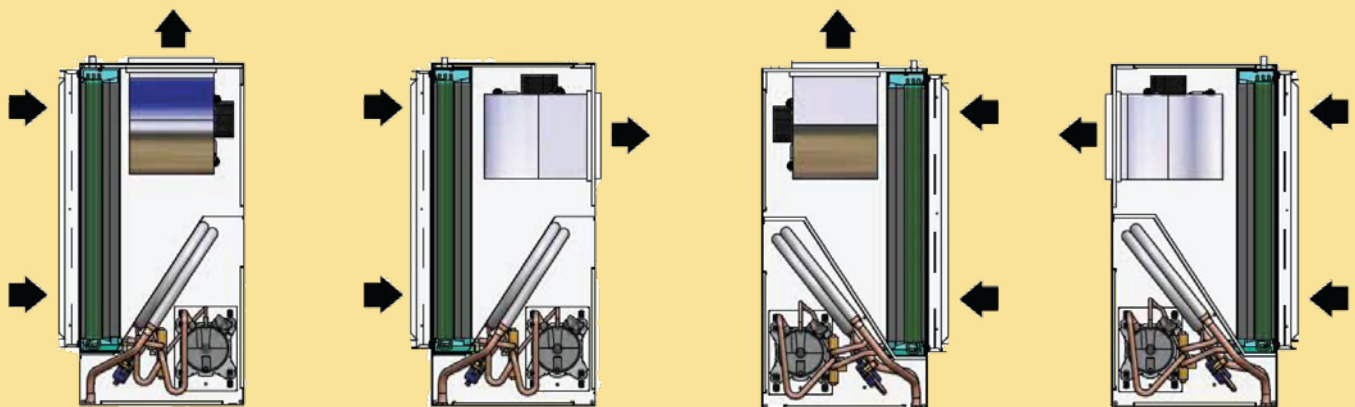
Left hand return with end discharge
